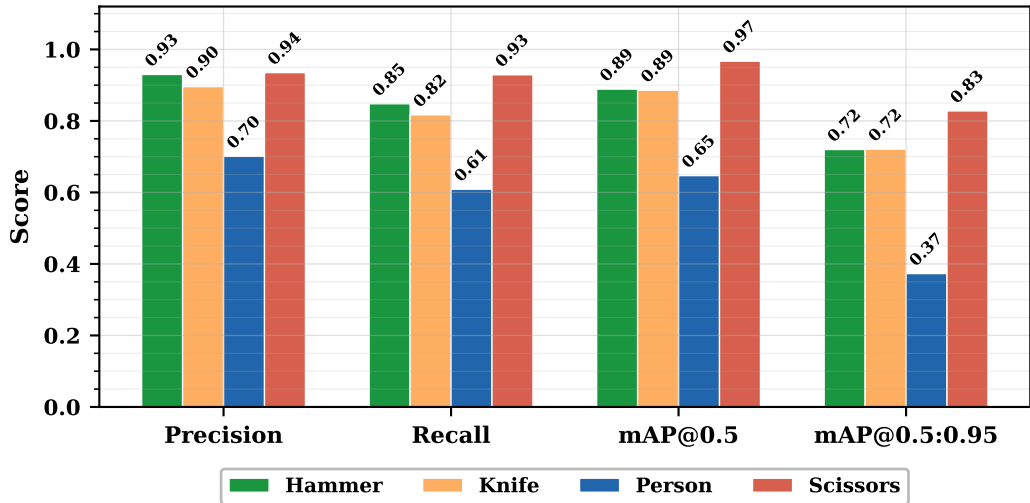
(a) Fine-tuned v5 (Final) — Per-Class Detection Performance (Test Set)
